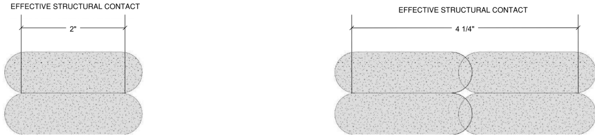
Figure 2: Effective width of wall sections
